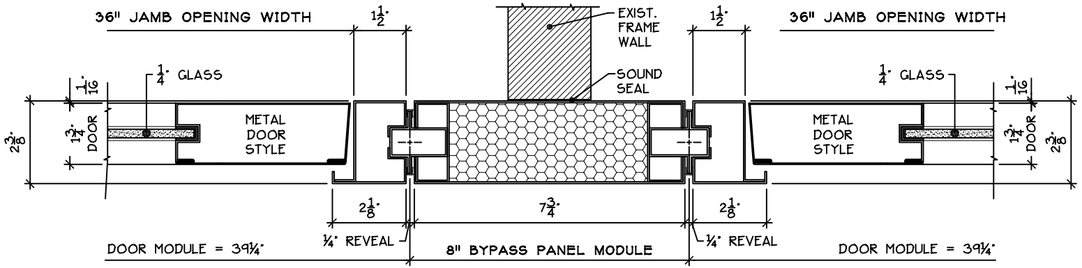
8" WALL BY-PASS PANEL AT DOOR FRAMES
