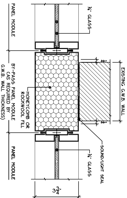
TYPICAL BY-PASS PANEL AT GLASS PANELS
