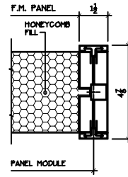
F.M. PANEL - FINISHED END POST
