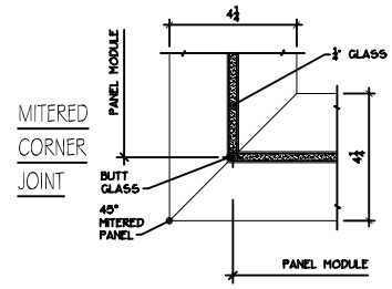
BUTT-END GLASS MITERED JOINT
