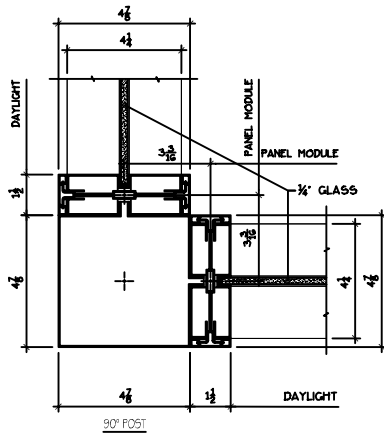
90° POST
