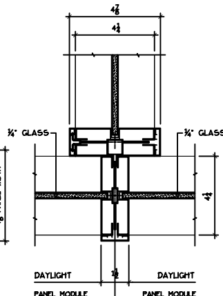
TEE POST 2
