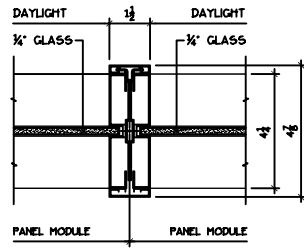
GLASS PANEL - INTERMEDIATE MULLION
