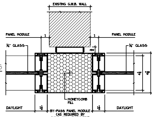
BY-PASS PANEL AT GLASS PANELS
