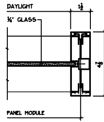
GLASS PANEL - FINISHED END POST
