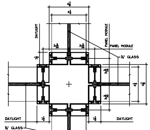
BUTT-END GLASS MITERED JOINT
