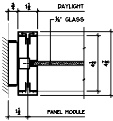
GLASS PANEL WALL STARTER
