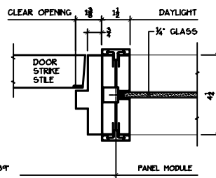
DOOR FRAME AT GLASS PANEL
