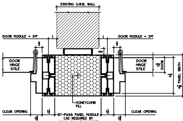
BY-PASS PANEL AT DOOR FRAMES
