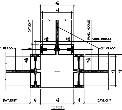
TEE POST 1
