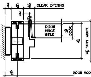
DOOR FRAME AT WALL START
