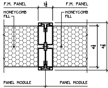
F.M. PANEL - INTERMEDIATE MULLION
