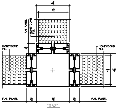
TEE POST I
