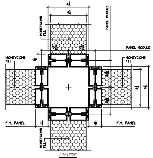
4-WAY POST
