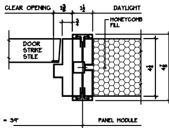
DOOR FRAME AT F.M. PANEL
