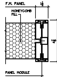
F.M. PANEL - FINISHED END POST
