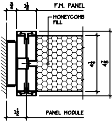
F.M. PANEL WALL STARTER
