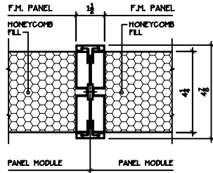
F.M. PANEL - INTERMEDIATE MULLION
