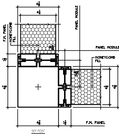
90° POST
