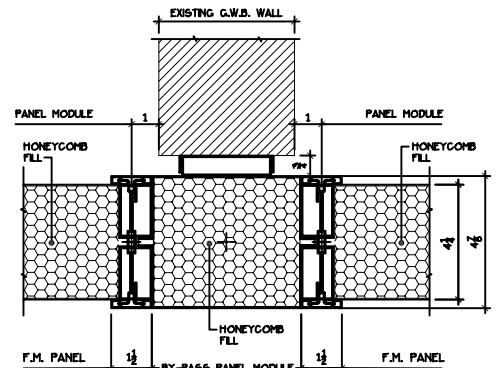
BY-PASS PANEL AT GLASS PANELS
